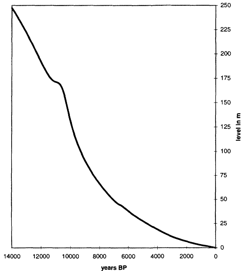
Figure 3-6. Graph showing the combined effect of the different glacio-isostatic movements used in the modelling. The parameters used for this calculation are A_1=200 m, T_1=12\,500 cal y BP, B_1=3800 , A_2=50 m, T_2=12\,000 cal y BP, B_2=-600 , A_3=50 m, T_3=11\,400 cal y BP and B_3=600 .
