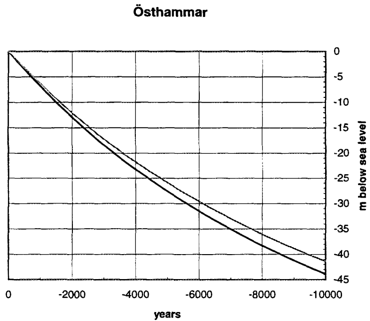
Figure 6-5. Predicted shore level displacement, grey curve, and the glacio-isostatic rise, black curve, at Östhammar in the county of Uppland. The uplift parameters used in the calculation are A_1 = 275 , B_1 = 8000 , A_3 = 80 , B_3 = 700 and T_3 = 10\,400 .
