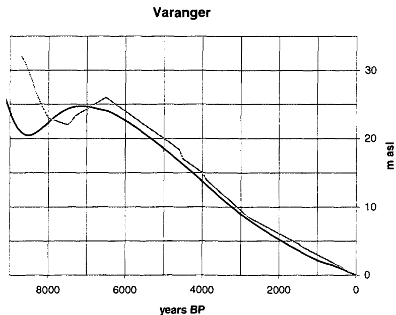
Figure 4-2. Site 1. Shore level displacement at the Varangerfjord according to Donner (1980), grey line. The calculated curve is black.
