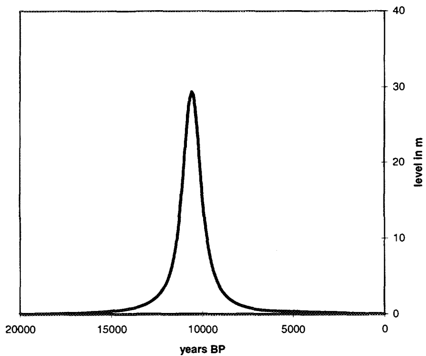
Figure 3-5. Graph of the combination of the crustal movements shown in Figures 3-3 and 3-4.
