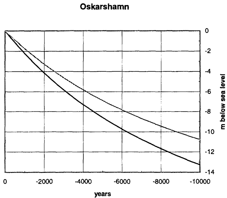
Figure 6-3. Predicted shore level displacement, grey curve, and the glacio-isostatic rise, black curve, at Oskarshamn, site 41. The uplift parameters used are in accordance with Table 5-1.
