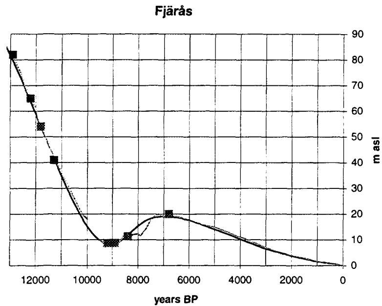
Figure 4-36. Site 34. Shore level displacement at Fjärås according to Pålse (1986).
