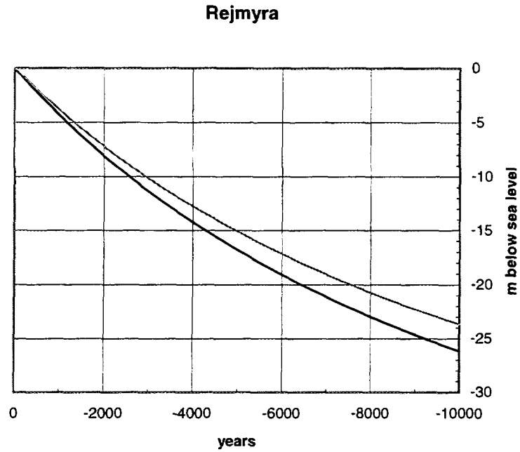
Figure 6-4. Predicted shore level displacement, grey curve, and the glacio-isostatic rise, black curve, at Rejmyra, site 43, W of Nyköping. The uplift parameters used are in accordance with Table 5-1.
