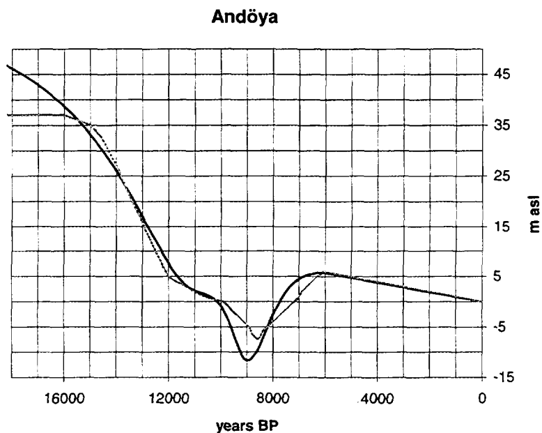
Figure 4-3. Site 2. Shore level displacement at Andöya according to Vorren et al. (1988). This area was unglaciated during the Late Weichselian and the original curve starts c. 18 000 years BP. The Holocene part of this curve is an interpolation of the curve shown at site 4. The calculated curve is somewhat too high between 18 000 - 16 000 years BP.
