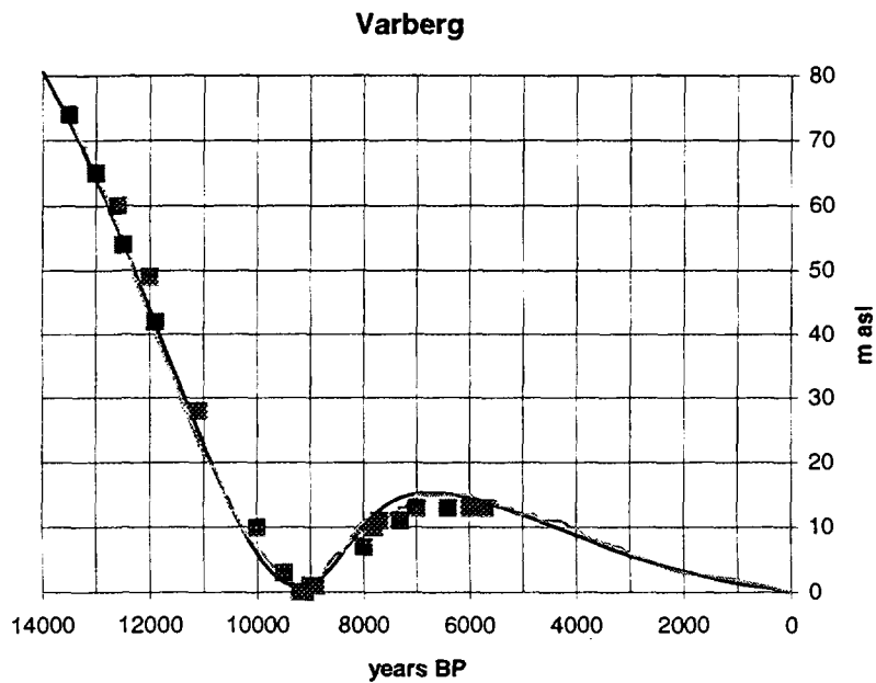
Figure 4-37. Site 35. Shore level displacement at Varberg according to Pålse (1990b). The data designated with squares in the Late Weichselian part is from Berglund (1995).
