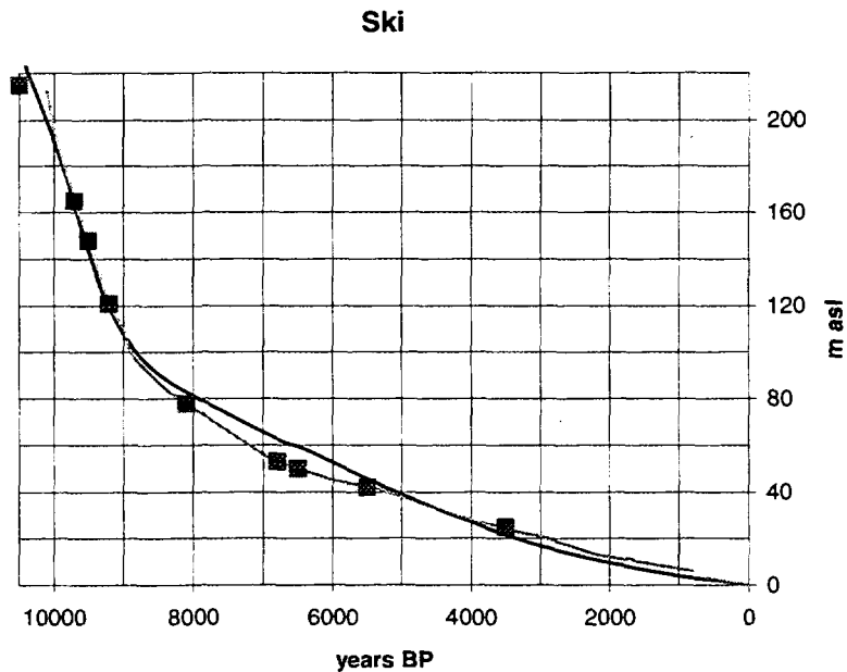
Figure 4-23. Site 22. Shore level displacement at Ski according to Sørensen (1979).
