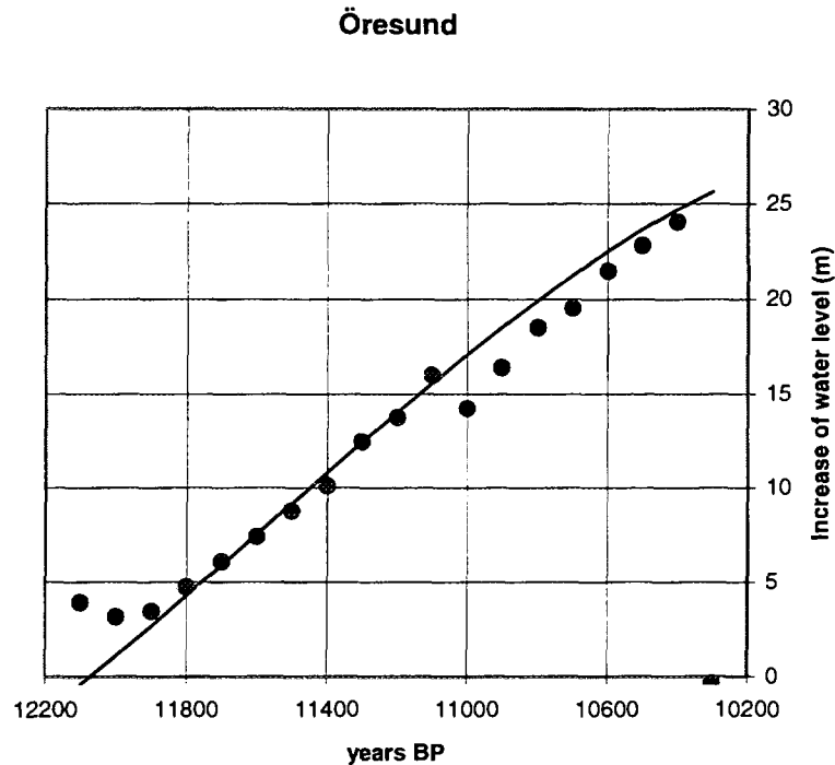
Figure 7-4. The water level rise in the Baltic Ice Lake. The water level rise recorded at Oskarshamn (site 41) is shown with dots. This rise is related to the calculated rate of shore level displacement at the threshold at Öresund, black line. The transgression in the Baltic Ice Lake continued to c. 10\,400 \pm 100 BP and reached a level of c. 26 m before the drainage.
