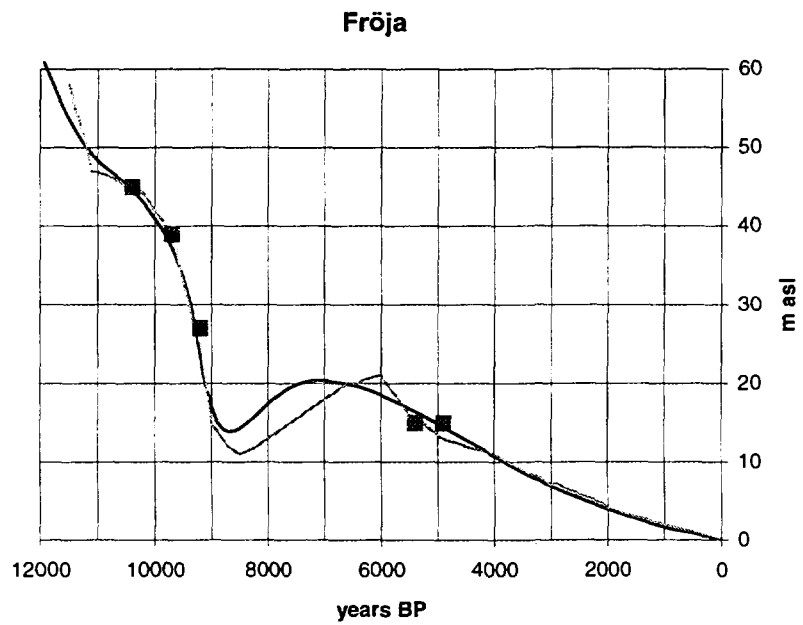
Figure 4-11. Site 10. Shore level displacement at Frøja according to Kjemperud (1986).
