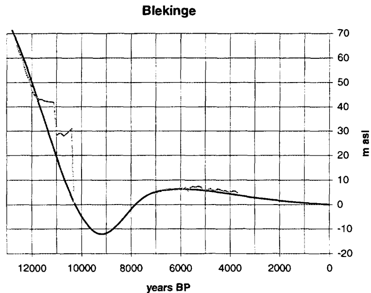
Figure 4-43. Site 40. Shore level displacement at Blekinge according to Björck (1979) and Liljegren (1982). The calculations indicate that the Baltic Ice Lake started to exist at c. 12 000 years BP.
