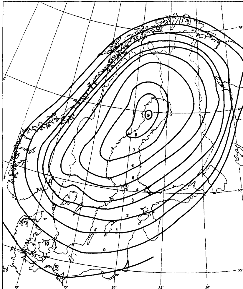
Figure 2-1. The recent relative uplift, v_r (mm/ y), recorded by precision levellings and tide gauge data. The map is redrawn from Ekman (1996).
