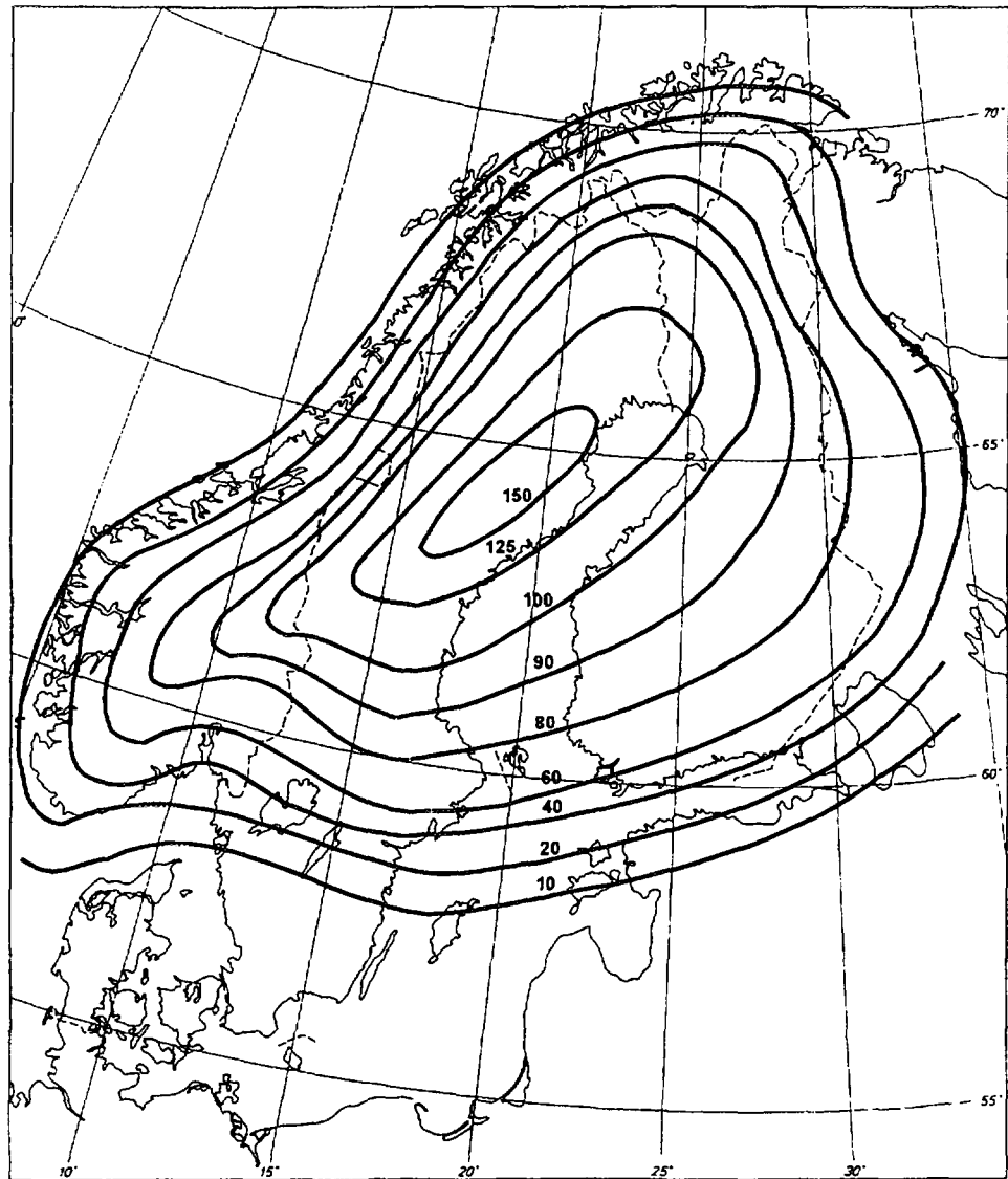
Figure 5-3. The values of A_3 (m), i.e. half of the total uplift for the fast uplift mechanism.
