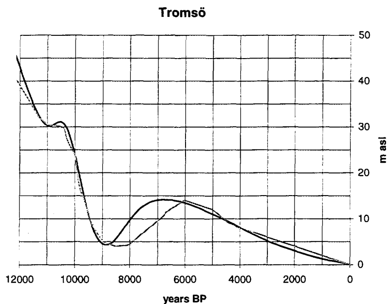
Figure 4-4. Site 3. Shore level displacement at Tromsø according to Hald & Vorren (1983). The shore level curve for Tromsø is based on modern data in the Late Weichselian- Preboreal part but relies on unmodern data for the Tapes transgression.
