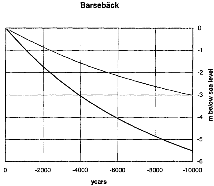
Figure 6-2. Predicted shore level displacement, grey curve, and the glacio-isostatic rise, black curve, at Barsebäck, site 39. The uplift parameters used are in accordance with Table 5-1.
