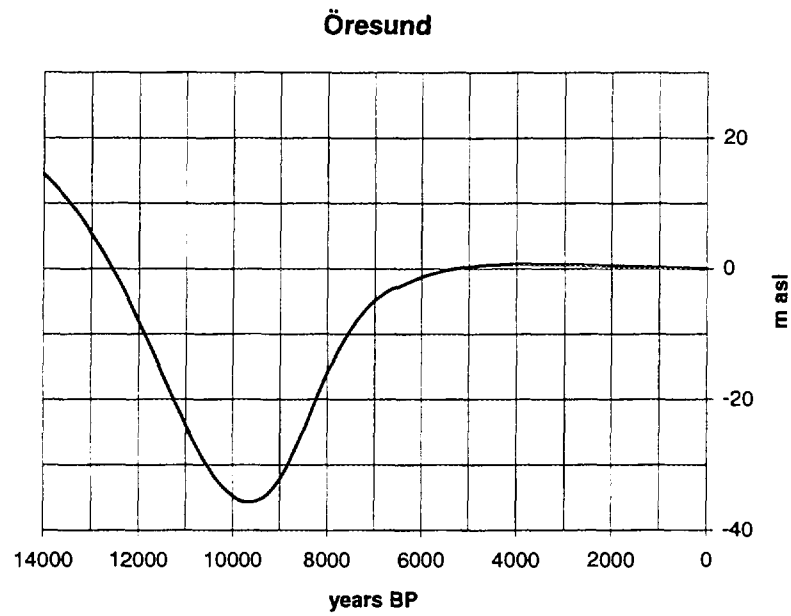
Figure 7-2. Shore level displacement at the Öresund Strait calculated with A_1 = 72 and B_1 = 2\,500 . The threshold at c. -7 was isolated c. 12 000 BP.
