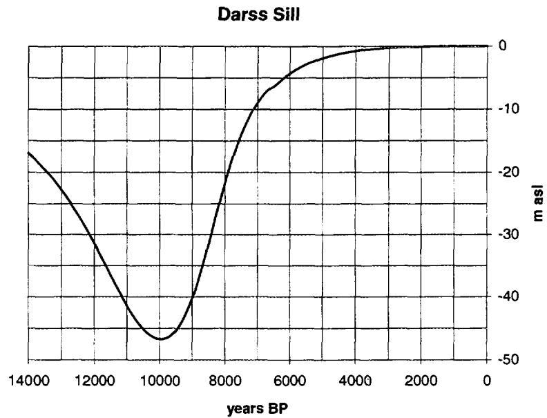
Figure 7-3. Shore level displacement at the Darss Sill calculated with A_1 = 50 and B_1 = 2\,500 . The threshold at c. -20 was isolated c. 13 500 BP.
